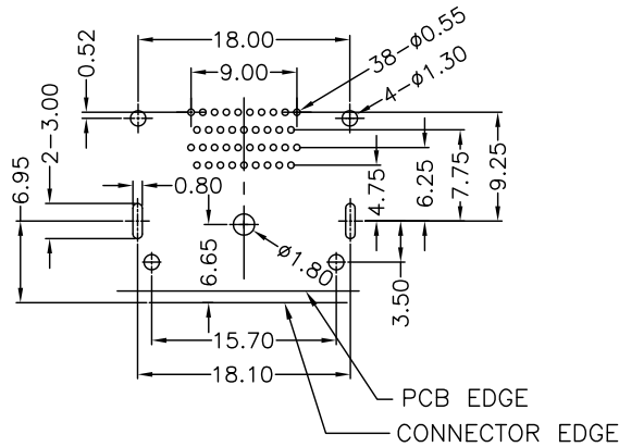
RECOMMEND P.C.B. LAYOUT TOLERANCE: ±0.05mm (TOP VIEW)
