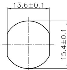
PG9 RECOMMENDED PANEL CUT-OUT THICKNESS 4.0 MAX.
