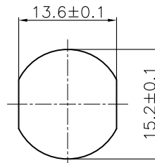
M15 RECOMMENDED PANEL CUT-OUT THICKNESS 4.0 MAX.
