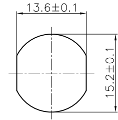
M15 RECOMMENDED PANEL CUT-OUT THICKNESS 4.0 MAX.
