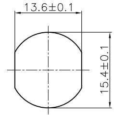
PG9 RECOMMENDED PANEL CUT-OUT THICKNESS 4.0 MAX.
