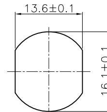
M16 RECOMMENDED PANEL CUT-OUT THICKNESS 4.0 MAX.
