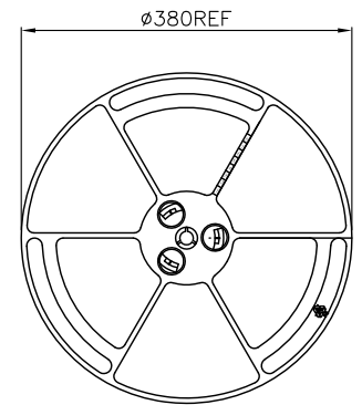
REEL FOR CARRIER TAPE
