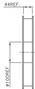
REEL FOR CARRIER TAPE
