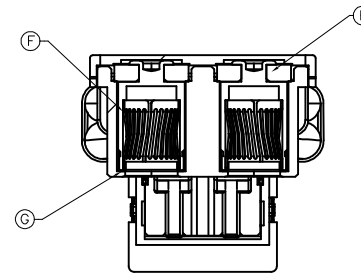
SECTION E-E SCALE 2:1
